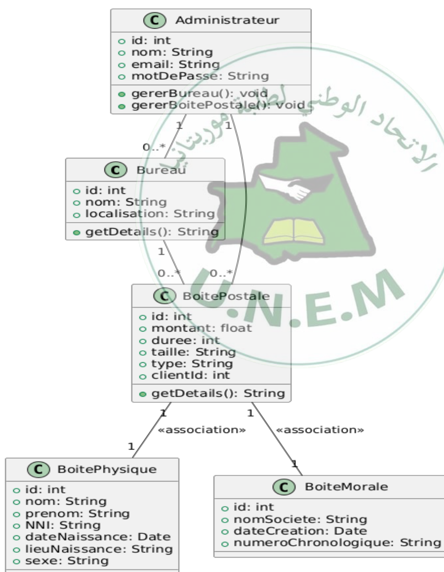
Figure 10: Diagramme de class
